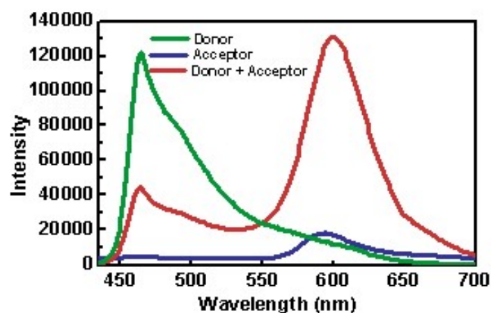
Figure 3: Fluorescence spectra of individual donor and acceptor and the mixed solution of donor and acceptor. Here the acceptor fluorescence increases by almost six times in presence of donor. Where as the donor fluorescence becomes one third of the individual donor fluorescence. This ratiometric change in fluorescence intensity is compelling visual evidence of FRET. The fluorescence spectra were recorded by exciting the emission maximum of the donor. [Here the fluorophore used are 3-octadecyl-2-[3-octadecyl-2 (3H)-benzothiazolidene] methyl] benzothiazolium perchlorate (donor), Octadecyl rhodamine B (acceptor)].
