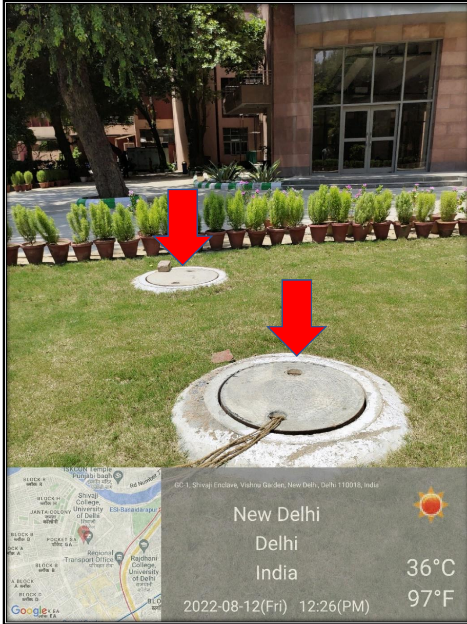
Roof-top Rainwater Harvesting Unit showing location of underground storage tank for storing (near Jijabai Academic Block)
